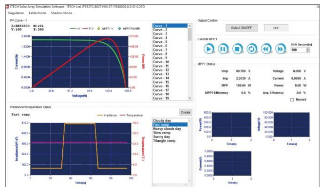
Simulation of I-V curves at different temperatures/irradiation
